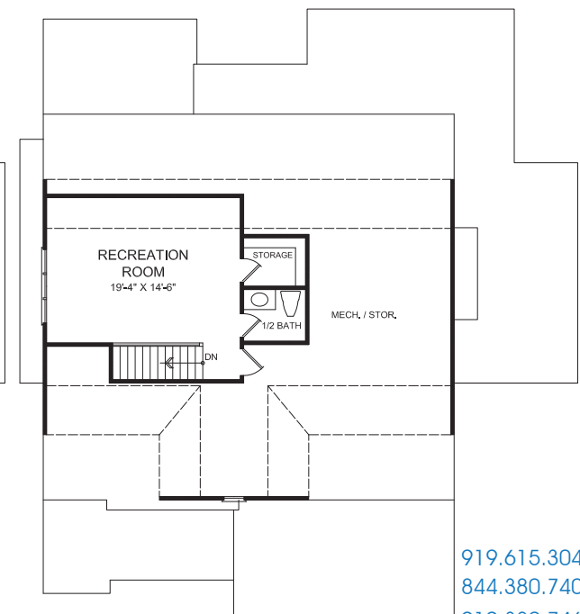
THIRD FLOOR
